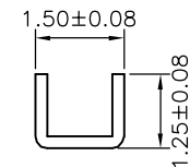
SEC:C-C
